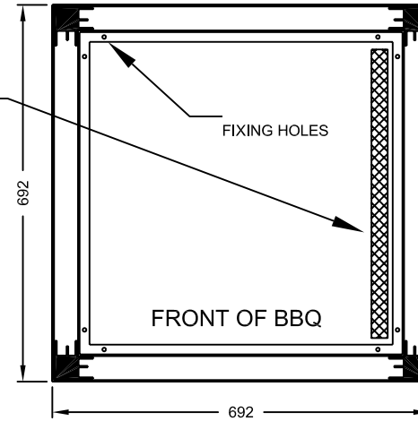
BASE DETAIL
