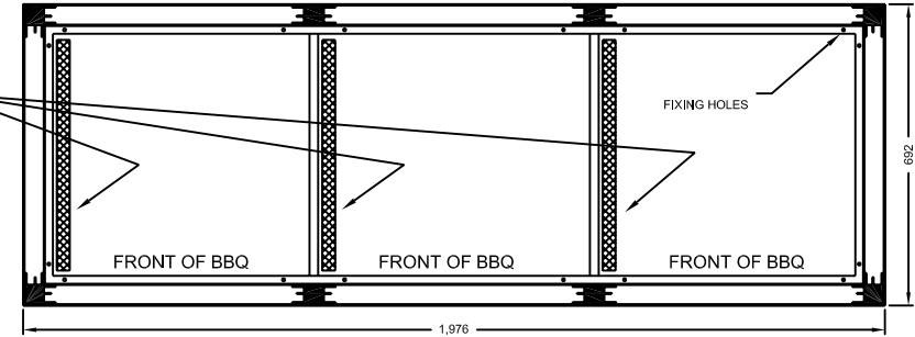
BASE DETAIL
