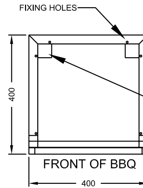
BASE DETAIL
